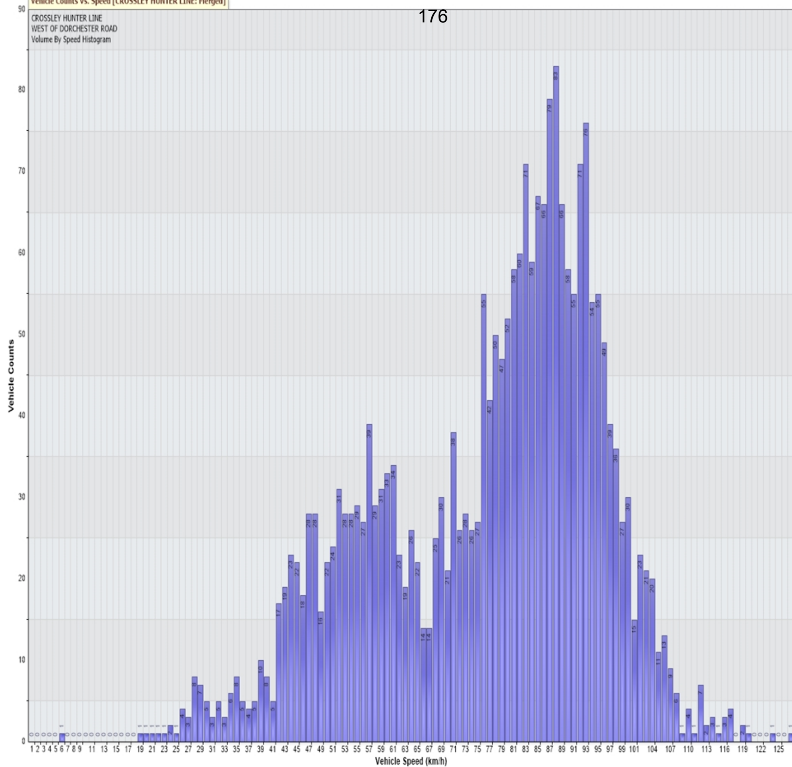
Vehicle Counts Vs. Speed [CROSSLEY HUNTER LINE: Merged]
