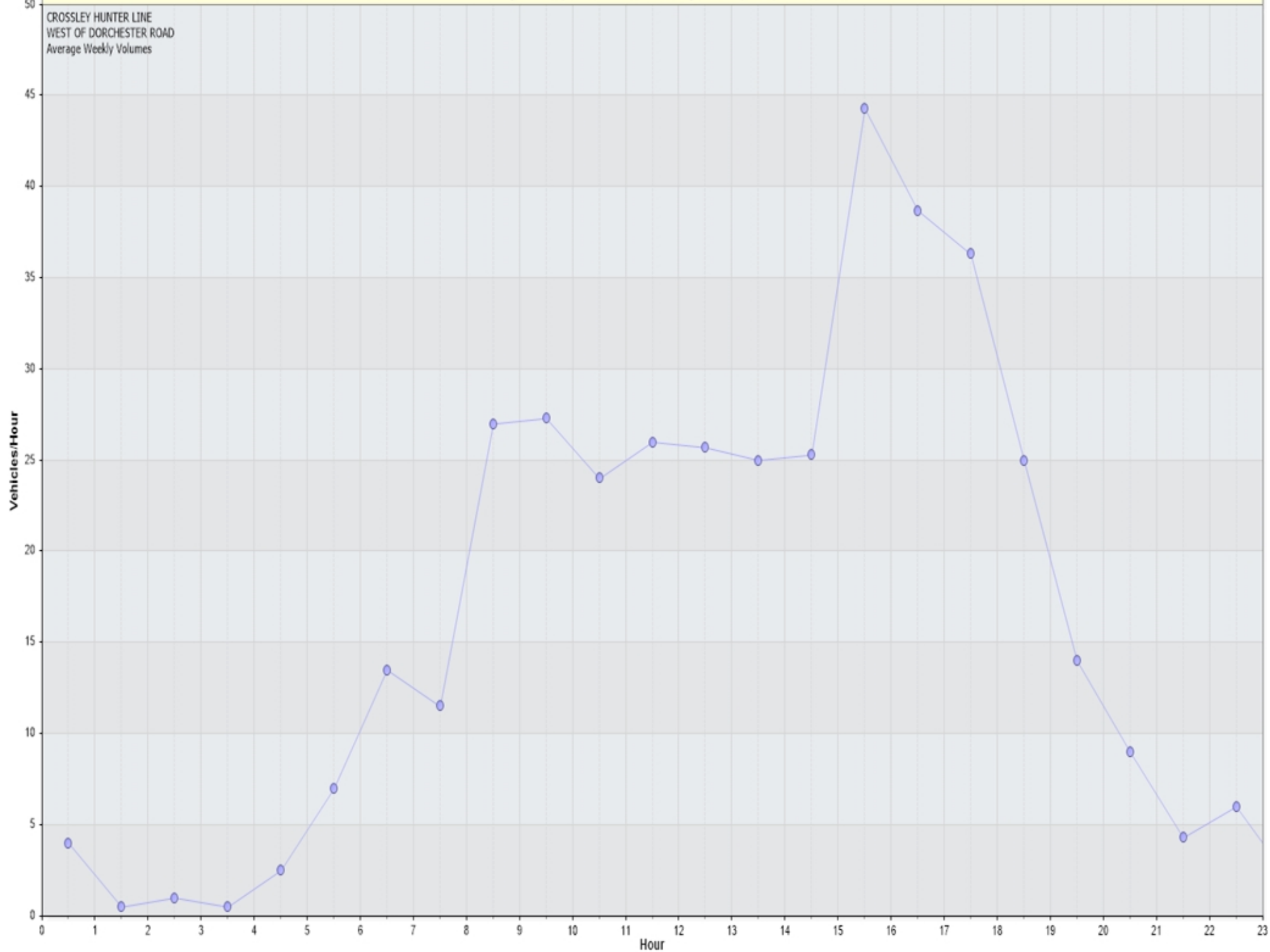
Merged: Average Hourly Volume for Week of 11/8/2021 Average Counts By Hour (11/8/2021) - Average Counts By Hour (11/8/2021)
