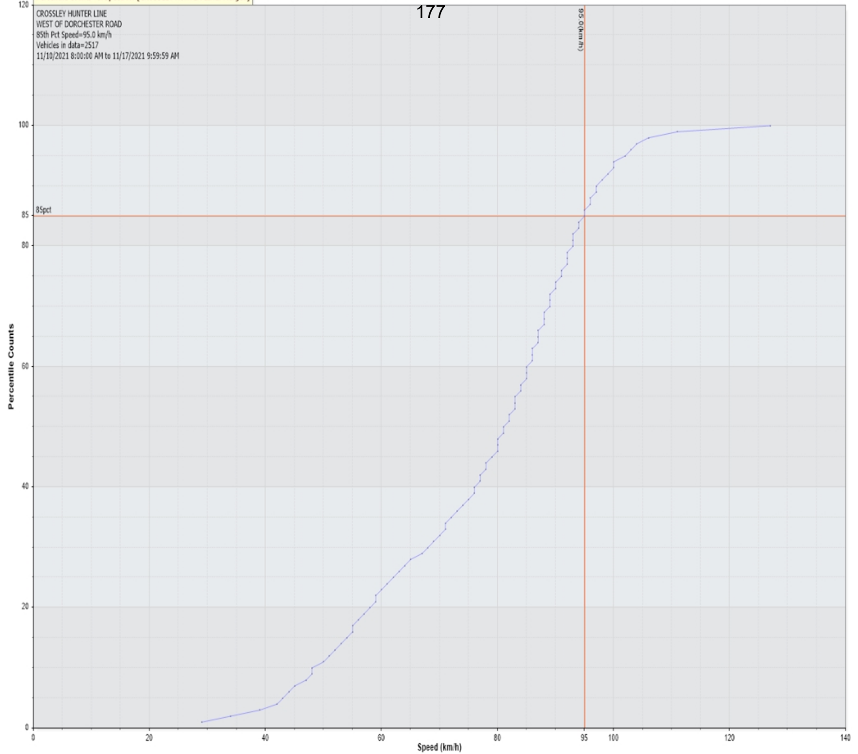
Percentile Counts Vs. Speed for [CROSSLEY HUNTER LINE: Merged]
