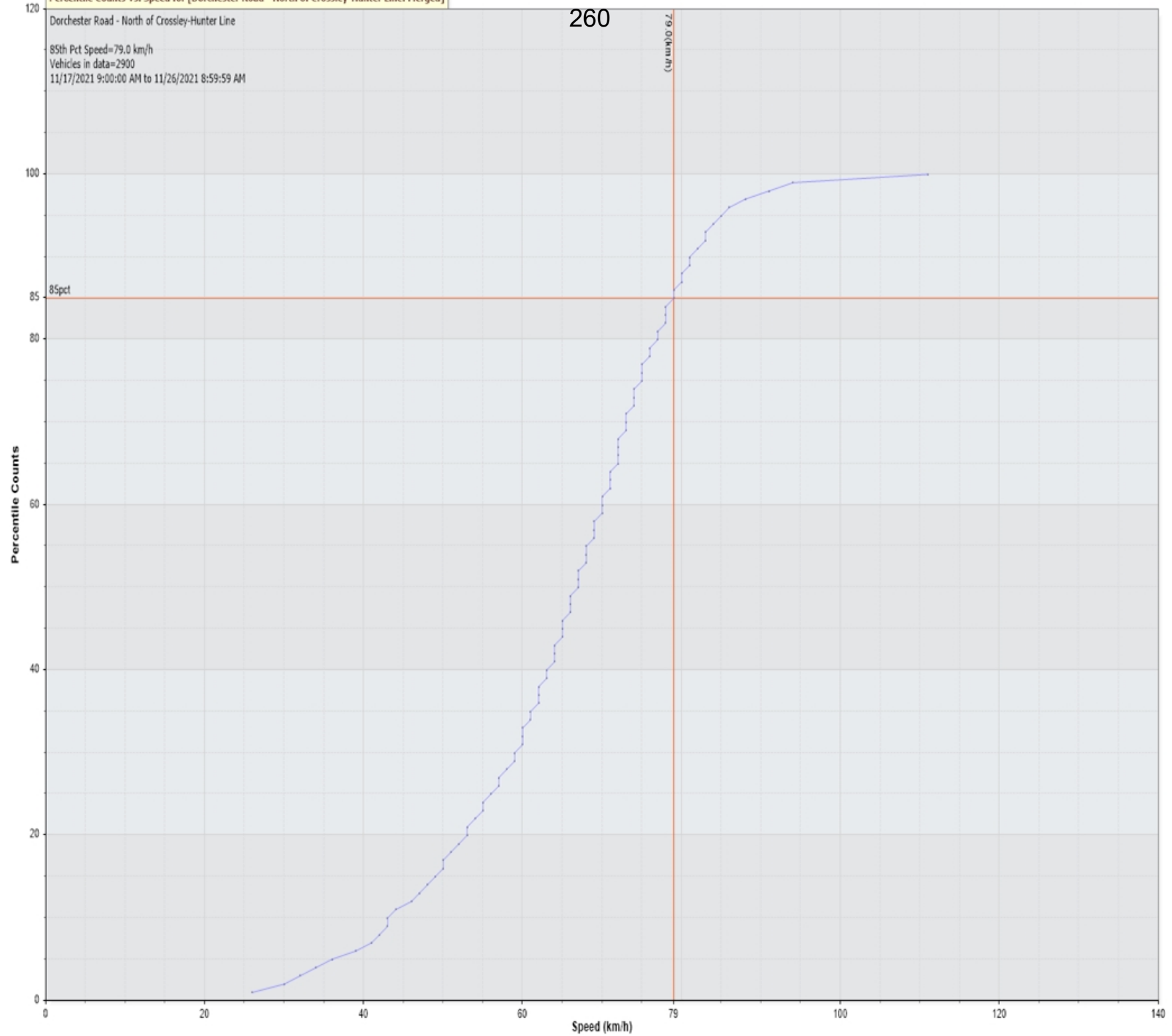
Percentile Counts Vs. Speed for [Dorchester Road - North of Crossley-Hunter Line: Merged]
