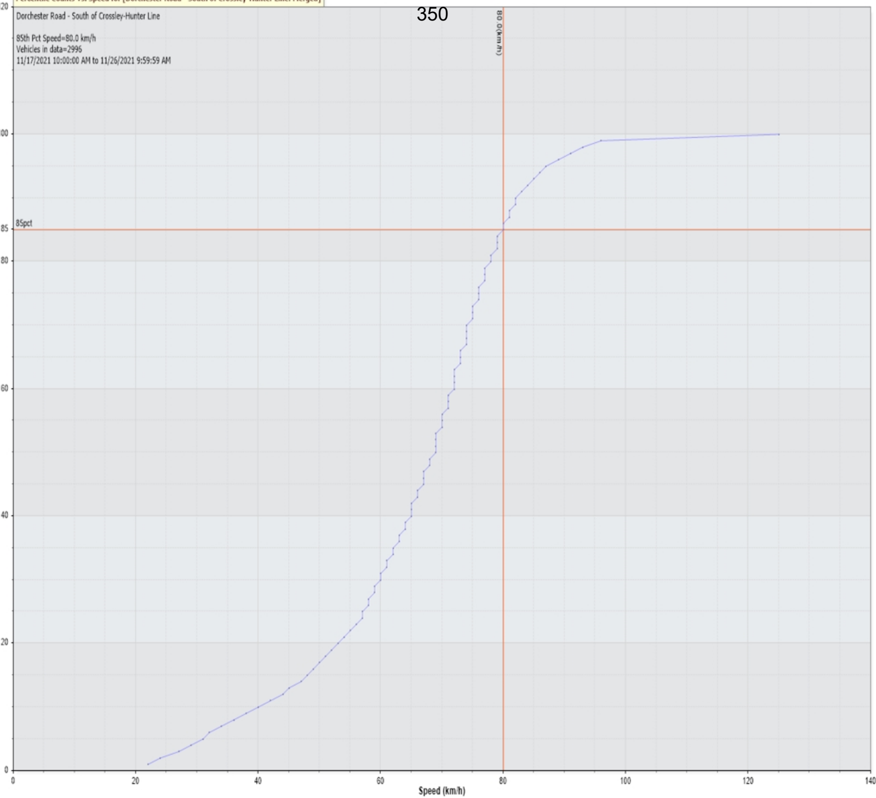
Percentile Counts Vs. Speed for [Dorchester Road - South of Crossley-Hunter Line: Merged]
