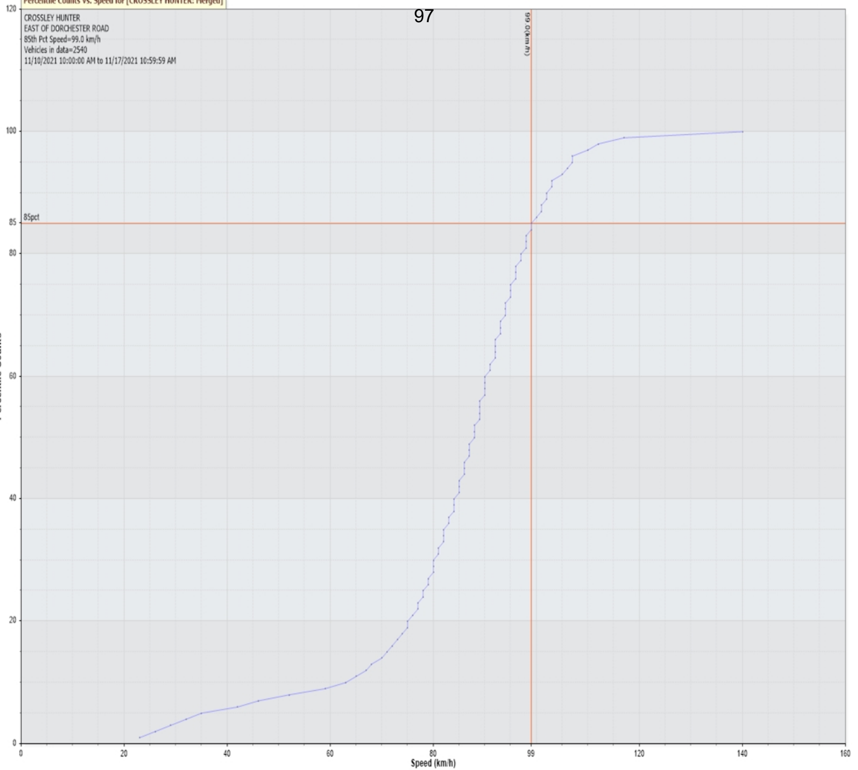
Percentile Counts Vs. Speed for [CROSSLEY HUNTER: Merged]
